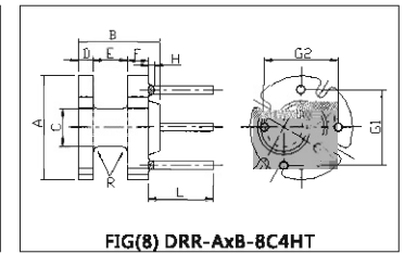
FIG(8) DRR-AxB-8C4HT
