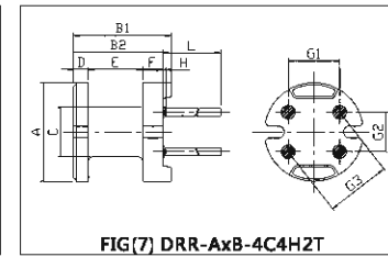
FIG(7) DRR-AxB-4C4H2T
